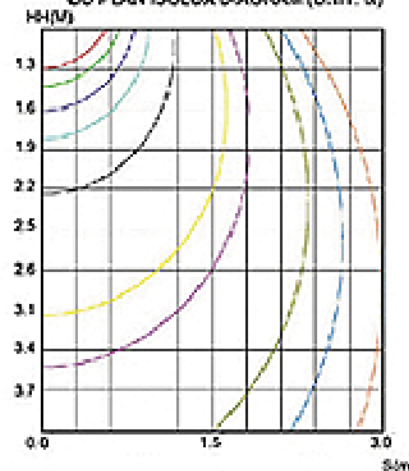
CO PLAN ISOLUX DIAGRAM (UNIT: lx)
